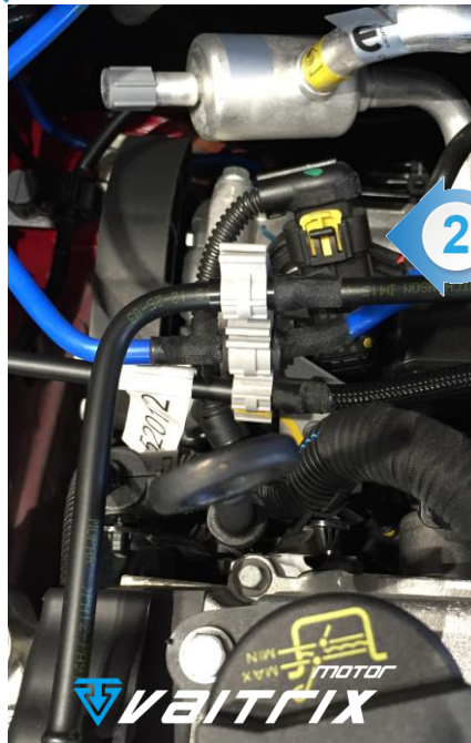
2 OP2 MANIFOLD (GAUGE)
