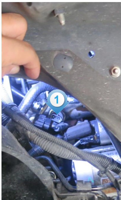
1 OP1 FUEL PRESSURE
