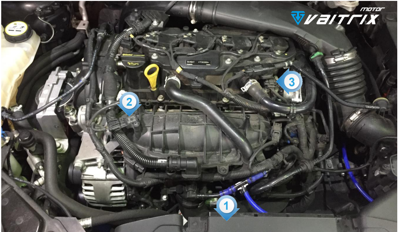
1 OP1 BOOST 2 OP2 MANIFOLD (GAUGE) 3 CAMSHAFT
